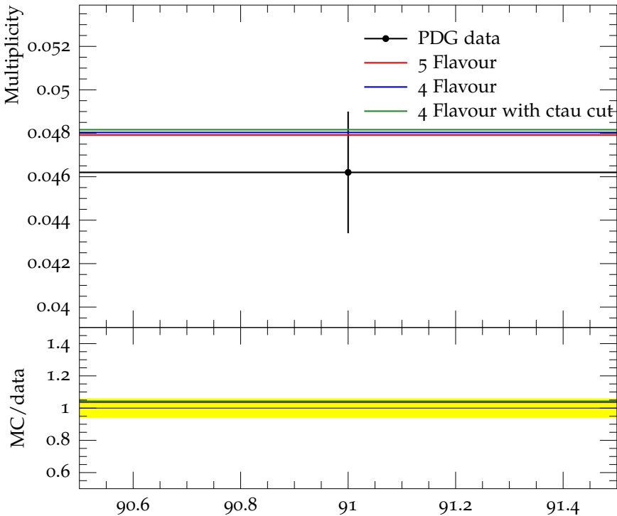
Mean \Sigma^\pm(1385) multiplicity
