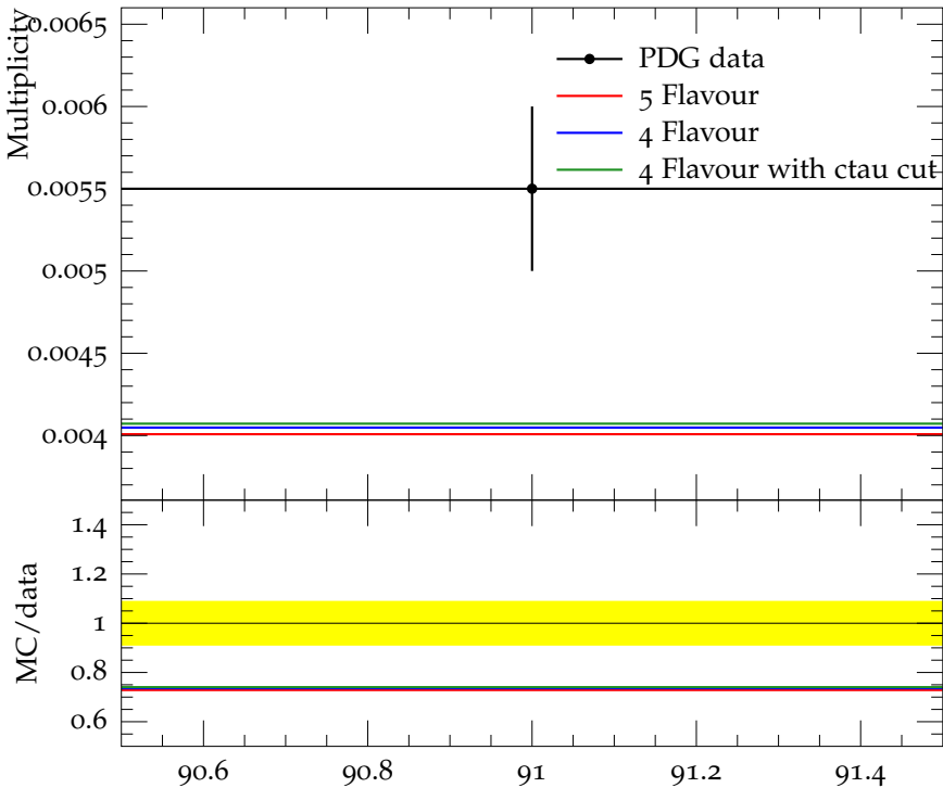
Mean \Xi^0(1530) multiplicity
