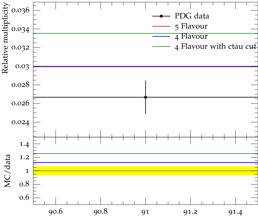
Ratio (w.r.t. \pi^\pm ) of mean D^0 multiplicity
