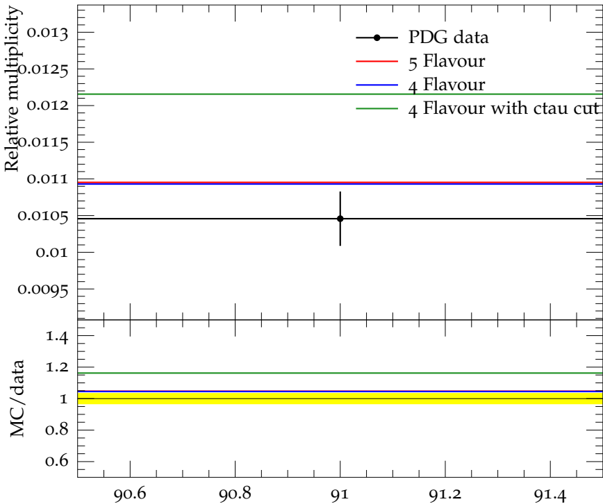
Ratio (w.r.t. \pi^\pm ) of mean B_u^+ multiplicity
