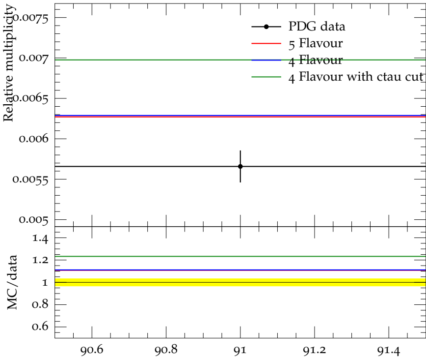
Ratio (w.r.t. \pi^\pm ) of mean \phi(1020) multiplicity
