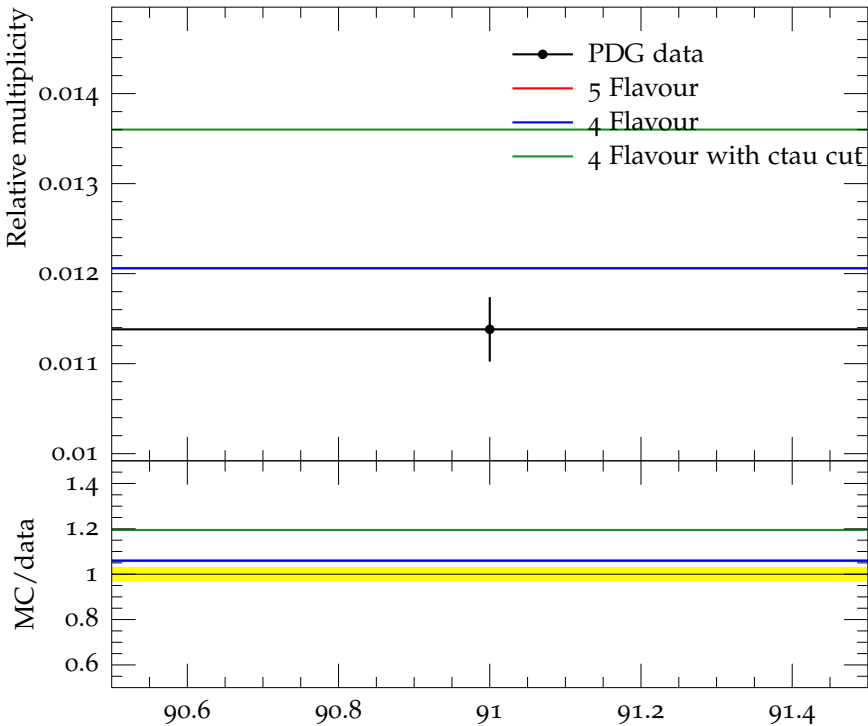
Ratio (w.r.t. \pi^\pm ) of mean D^{*+} (2010) multiplicity
