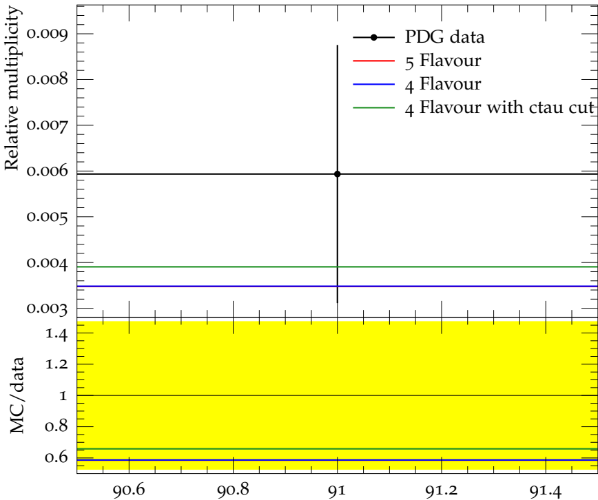
Ratio (w.r.t. \pi^\pm ) of mean D_s^{*+}(2112) multiplicity
