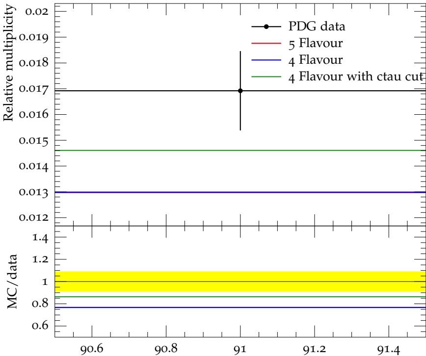
Ratio (w.r.t. \pi^\pm ) of mean B^* multiplicity
