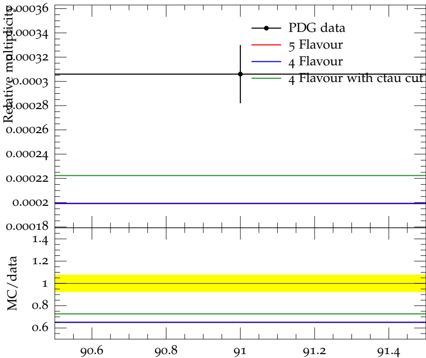
Ratio (w.r.t. \pi^\pm ) of mean J/\psi(1S) multiplicity
