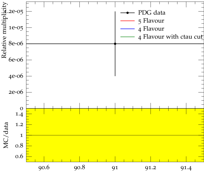
Ratio (w.r.t. \pi^\pm ) of mean Y(1S) multiplicity
