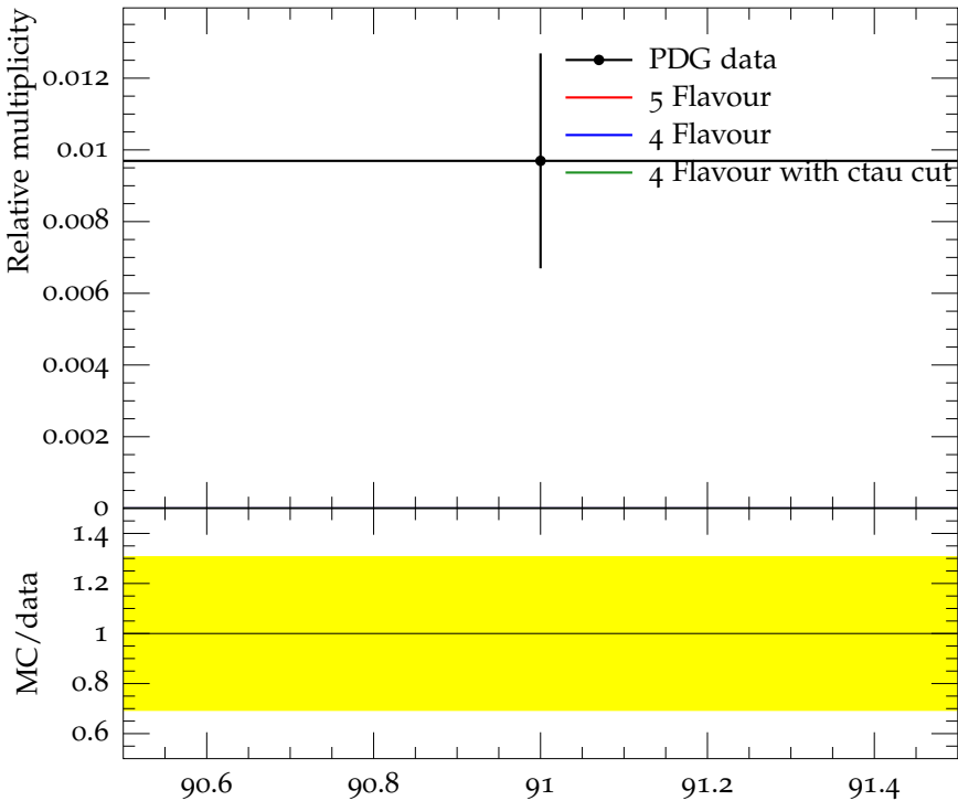
Ratio (w.r.t. \pi^\pm ) of mean f_1(1285) multiplicity
