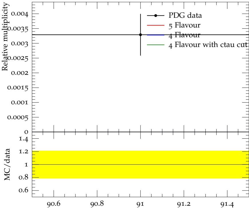
Ratio (w.r.t. \pi^\pm ) of mean f_1(1420) multiplicity
