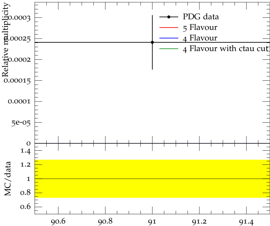
Ratio (w.r.t. \pi^\pm ) of mean \chi_{c1}(3510) multiplicity
