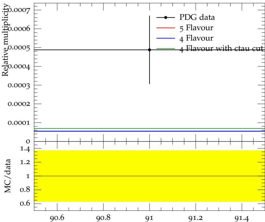
Ratio (w.r.t. \pi^\pm ) of mean D_{s2}^+ multiplicity
