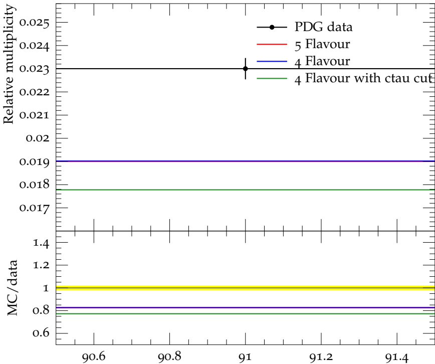
Ratio (w.r.t. \pi^\pm ) of mean \Lambda multiplicity
