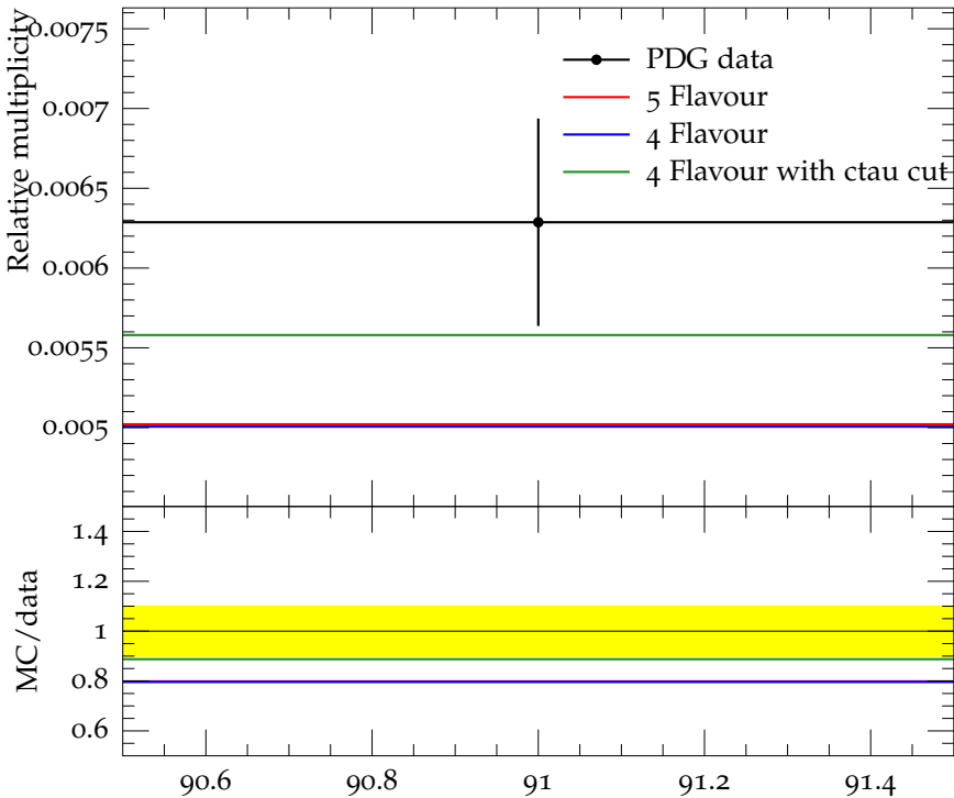
Ratio (w.r.t. \pi^\pm ) of mean \Sigma^+ multiplicity
