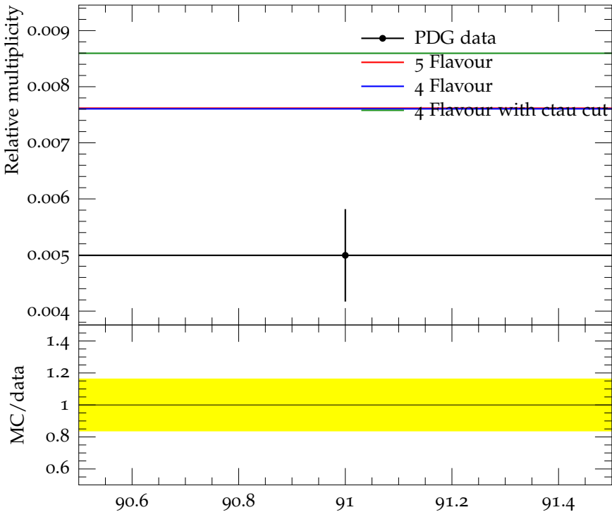
Ratio (w.r.t. \pi^\pm ) of mean \Delta^{++}(1232) multiplicity
