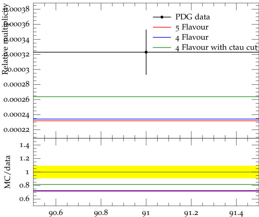
Ratio (w.r.t. \pi^\pm ) of mean \Xi^0(1530) multiplicity
