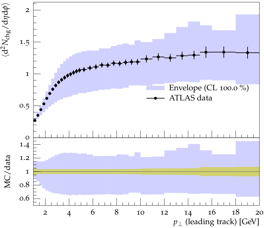
Toward N_{\text{chg}} density vs. p_{\perp}^{\text{trk1}} , \sqrt{s} = 7 TeV
