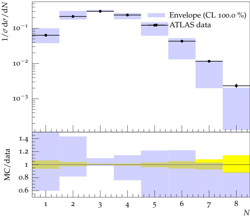
Charged jet multiplicity (anti- k_t , R = 0.4 , y 0.0-0.5, p_\perp 4.0-6.0)
