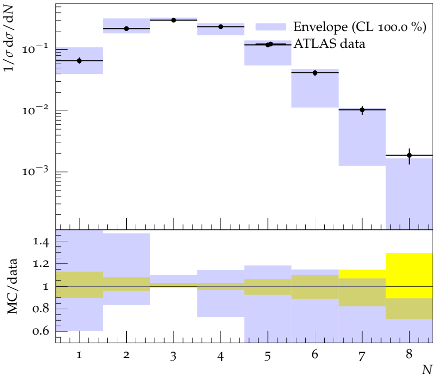
Charged jet multiplicity (anti- k_t , R = 0.4 , y 1.5-1.9, p_\perp 4.0-6.0)
