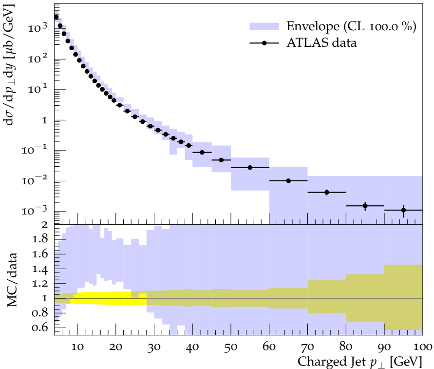
Charged jet cross section vs. p_{\perp} (anti- k_t , R = 0.6 , y 1.0-1.5)
