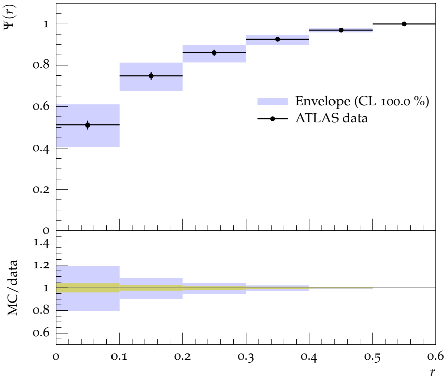
Jet shape \Psi for p_{\perp} \in 60\text{--}80\text{ GeV} , y \in 0.0\text{--}0.3
