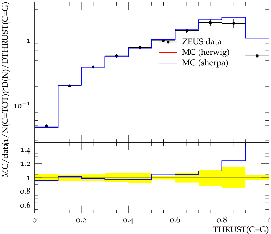
Differential Distribution of Thrust( C=G )
