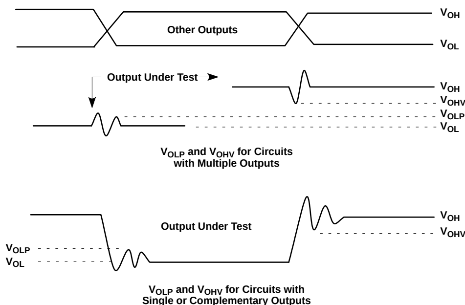
Figure 1. Test Waveforms
