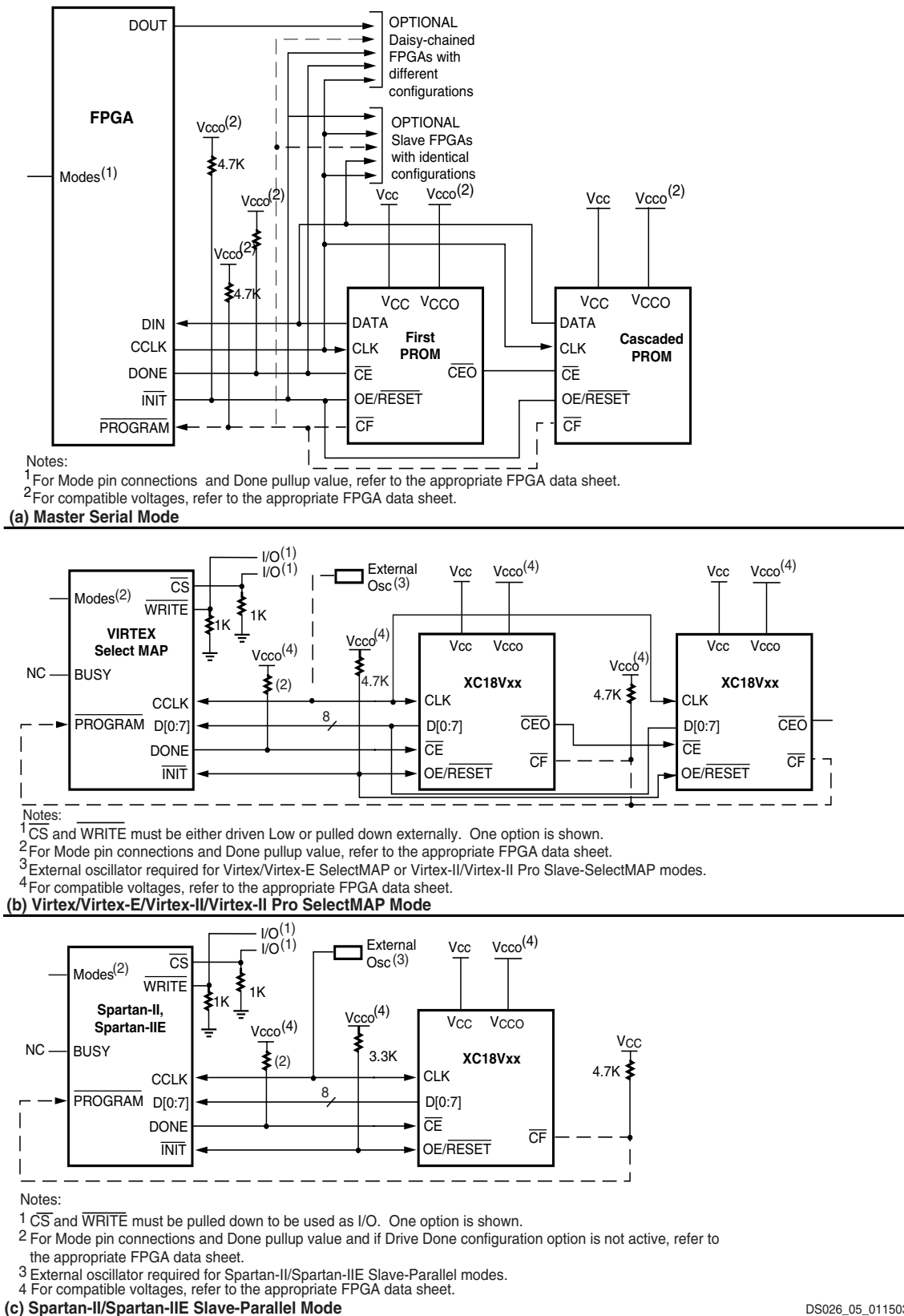
Figure 7: (a) Master Serial Mode (b) Virtex/Virtex-E/Virtex-II Pro SelectMAP Mode (c) Spartan-II/Spartan-IIE Slave-Parallel Mode (dotted lines indicate optional connection)
