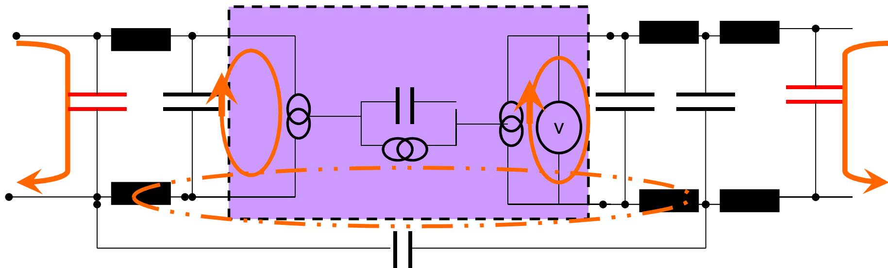
DC/DC converter: isolating version
