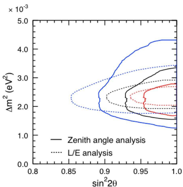
Figure 4: Allowed region for the atmospheric \Delta m^2 and mixing angle from the Super-Kamiokande experiment [6]. The solid and dashed curves come from two different data analyses. For each analysis, the innermost, middle, and outermost curves bound the 68, 90, and 99% confidence level regions, respectively.
