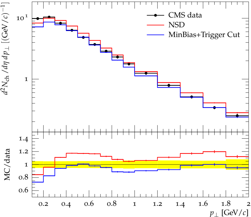
Charged hadron p_{\perp} for |\eta| = 1.3 at \sqrt{s} = 7 TeV
