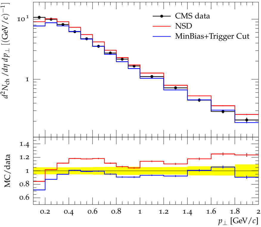
Charged hadron p_{\perp} for |\eta| = 2.3 at \sqrt{s} = 7 TeV
