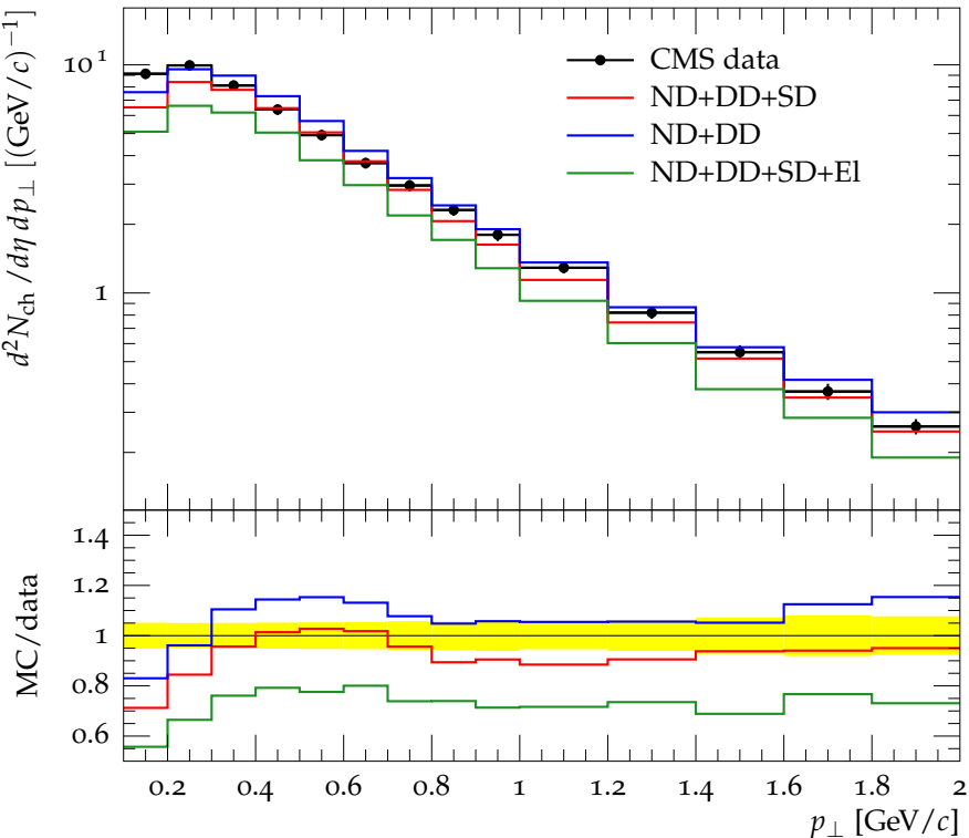
Charged hadron p_{\perp} for |\eta| = 0.7 at \sqrt{s} = 7 TeV
