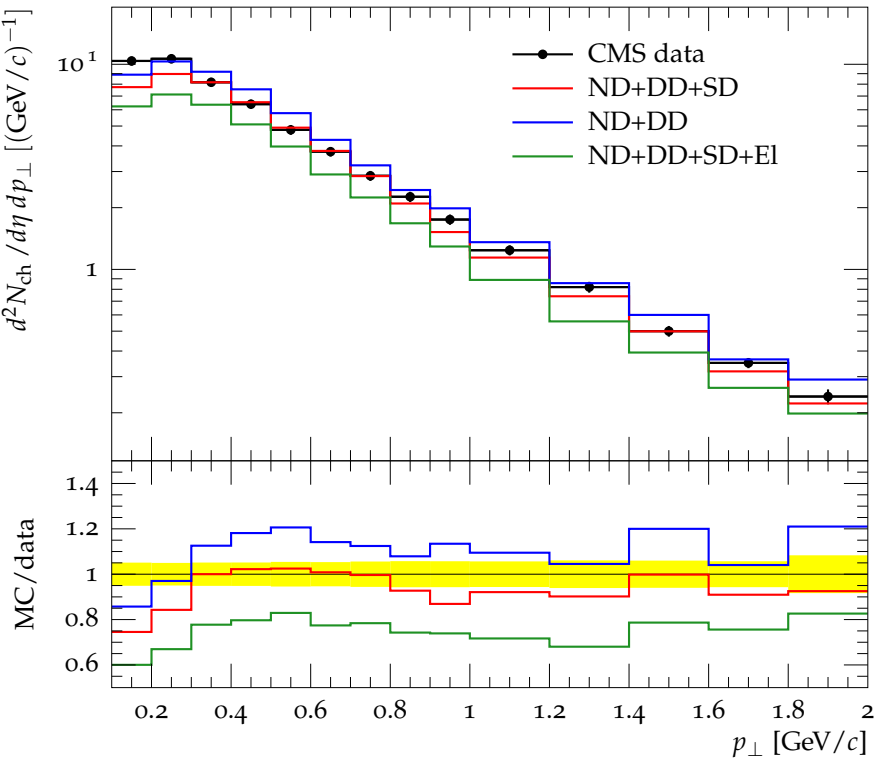
Charged hadron p_{\perp} for |\eta| = 1.7 at \sqrt{s} = 7 TeV
