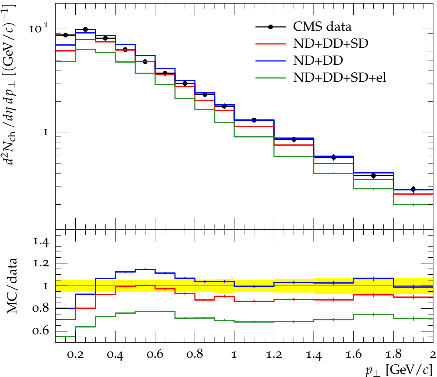
Charged hadron p_{\perp} for |\eta| = 0.5 at \sqrt{s} = 7 TeV
