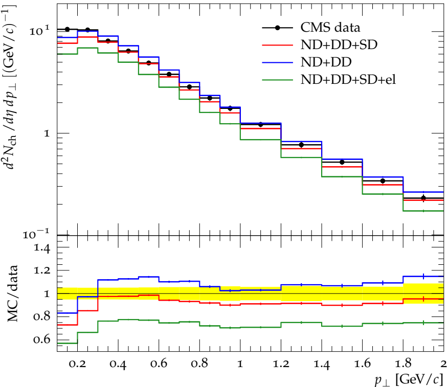
Charged hadron p_{\perp} for |\eta| = 1.9 at \sqrt{s} = 7 TeV
