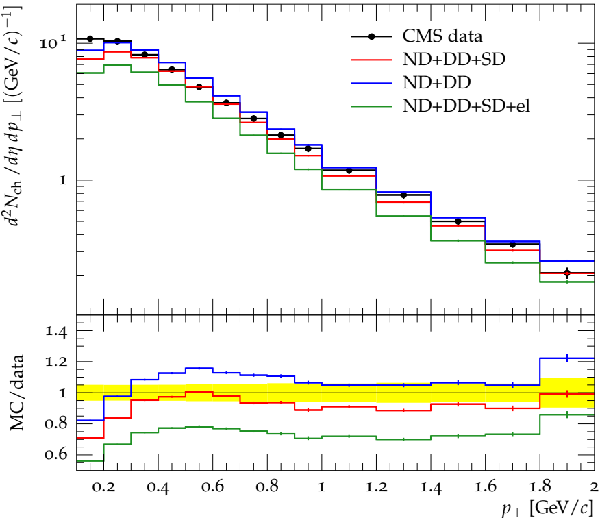
Charged hadron p_{\perp} for |\eta| = 2.1 at \sqrt{s} = 7 TeV
