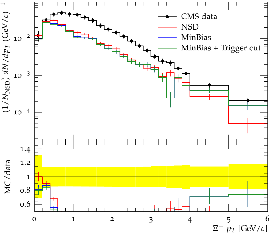
\Xi^- transverse momentum distribution at \sqrt{s} = 7 TeV
