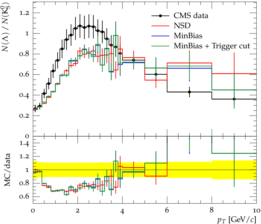
\Lambda/K_S^0 versus transverse momentum at \sqrt{s} = 7 TeV
