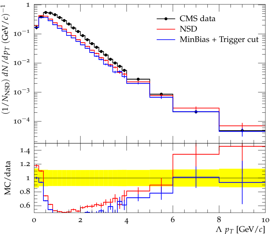
\Lambda transverse momentum distribution at \sqrt{s} = 7 TeV
