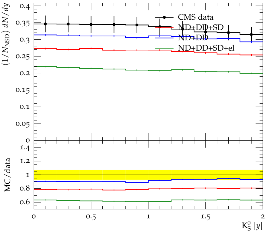
K_S^0 rapidity distribution at \sqrt{s} = 7 TeV
