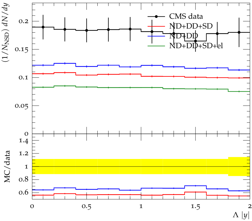
\Lambda rapidity distribution at \sqrt{s} = 7 TeV
