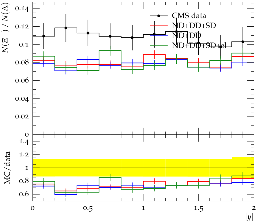
\Xi^- / \Lambda versus rapidity at \sqrt{s} = 7 TeV
