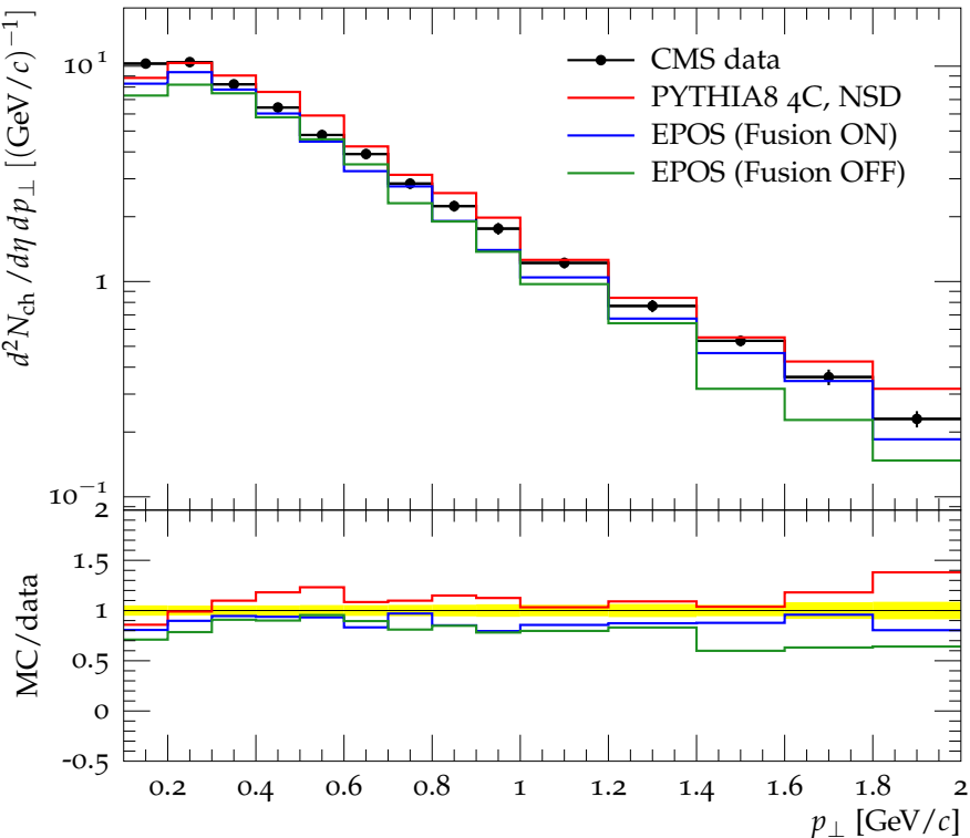
Charged hadron p_{\perp} for |\eta| = 1.5 at \sqrt{s} = 7 TeV
