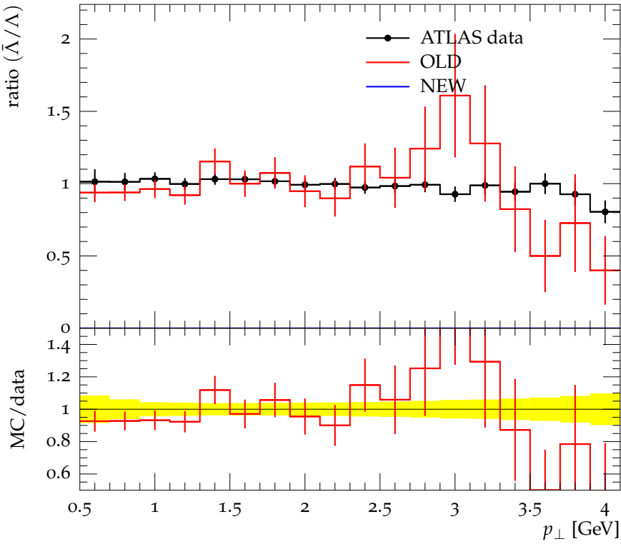
Production ratio of \bar{\Lambda} and \Lambda vs. p_{\perp} , \sqrt{s} = 7000 GeV
