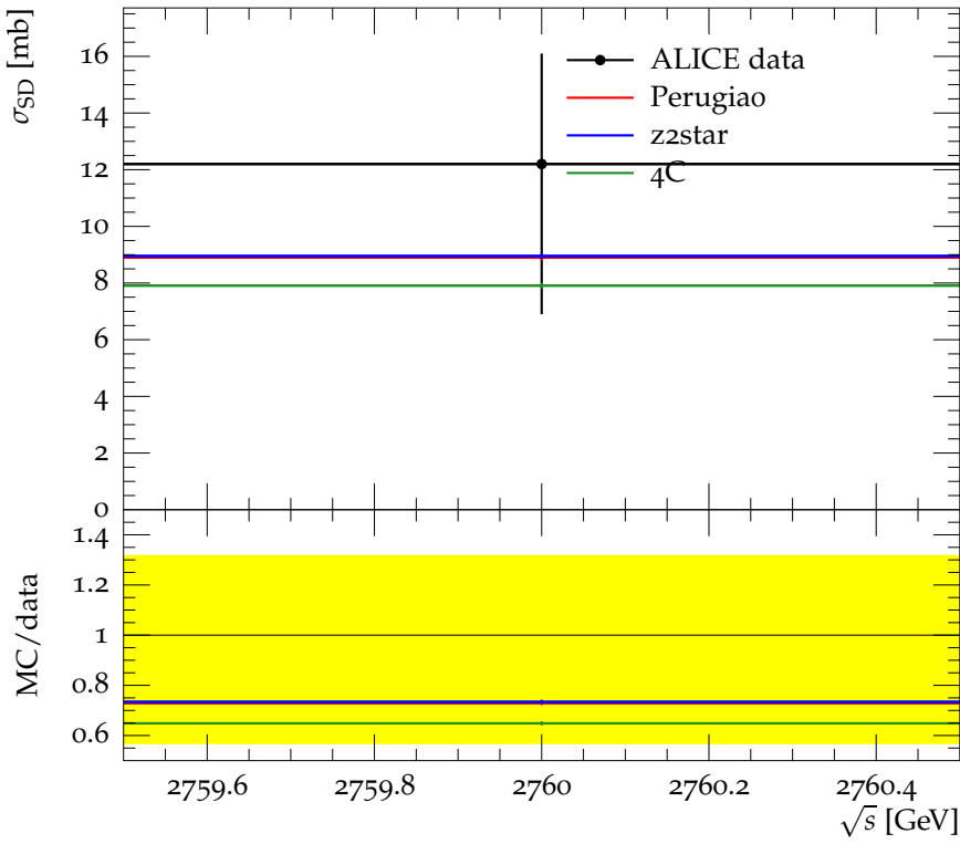
Single diffraction cross-section for M_X < 200 \text{ GeV}/c^2
