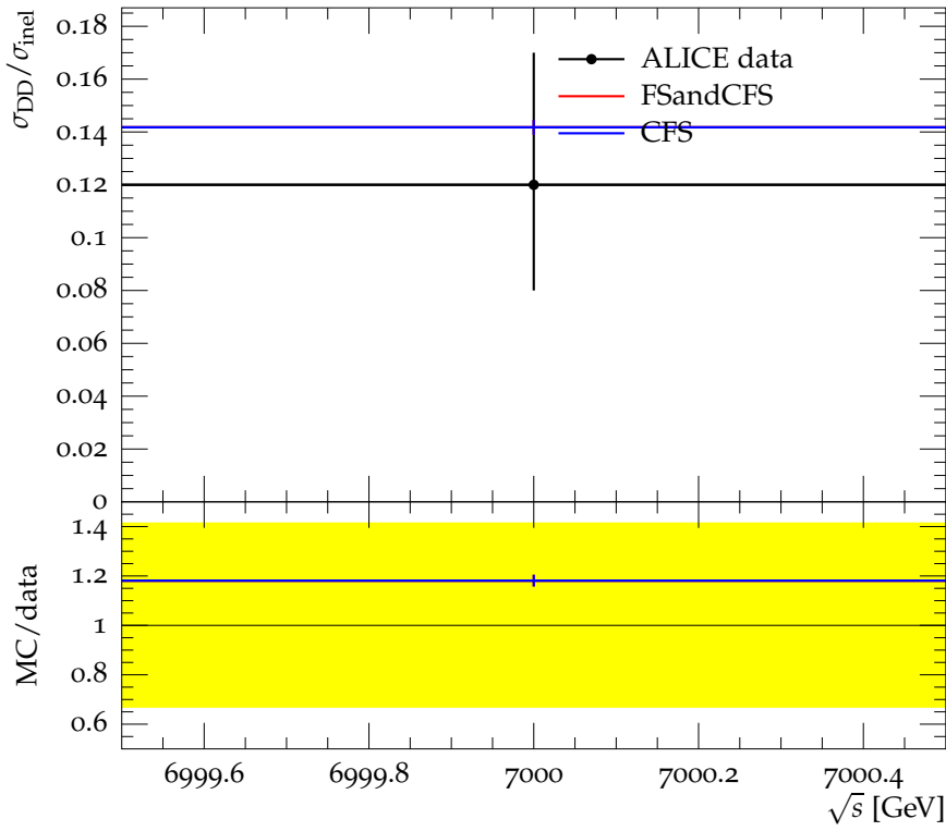
Production ratios of DD with \Delta\eta > 3 to INEL
