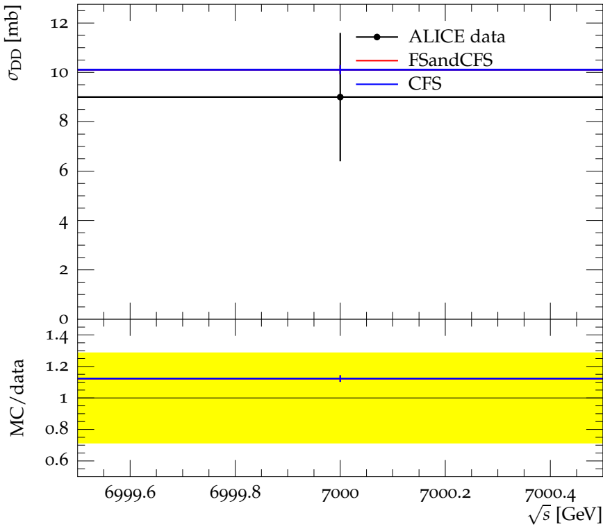
Double diffraction cross-section for \Delta\eta > 3
