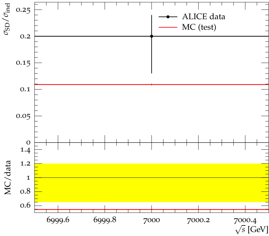
Production ratios of SD with M_X < 200 \text{ GeV}/c^2 to INEL
