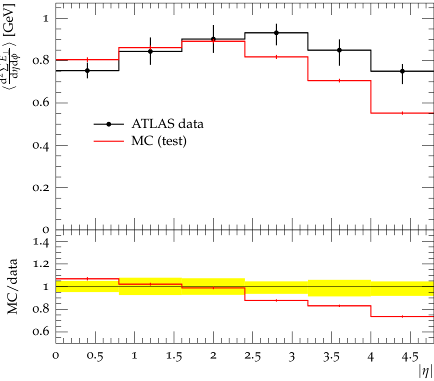
E_{\perp} density for the minimum bias selection
