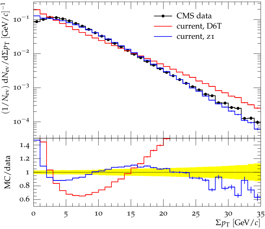
Distribution \Sigma p_T at 7 TeV, max p_T > 20 GeV/c
