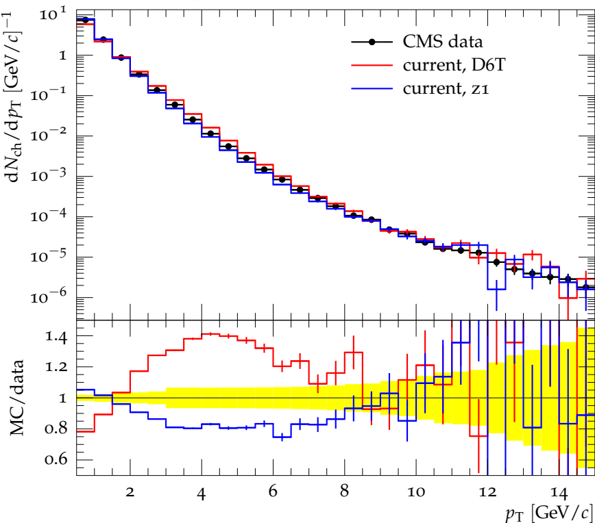
Distribution p_T at 7 TeV, max p_T > 20 GeV/c
